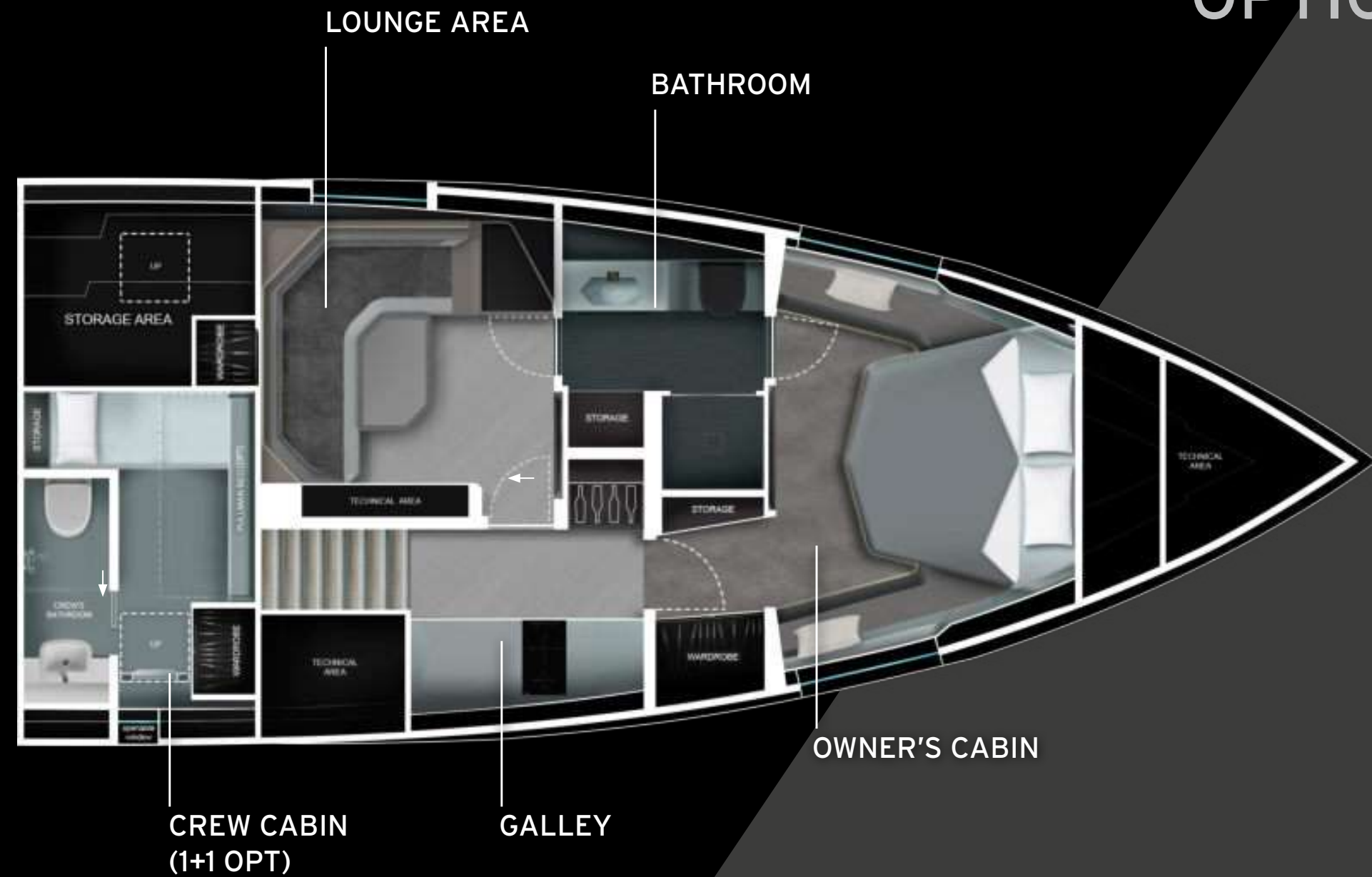
1 CABIN + 1 LOUNGE LAYOUT
