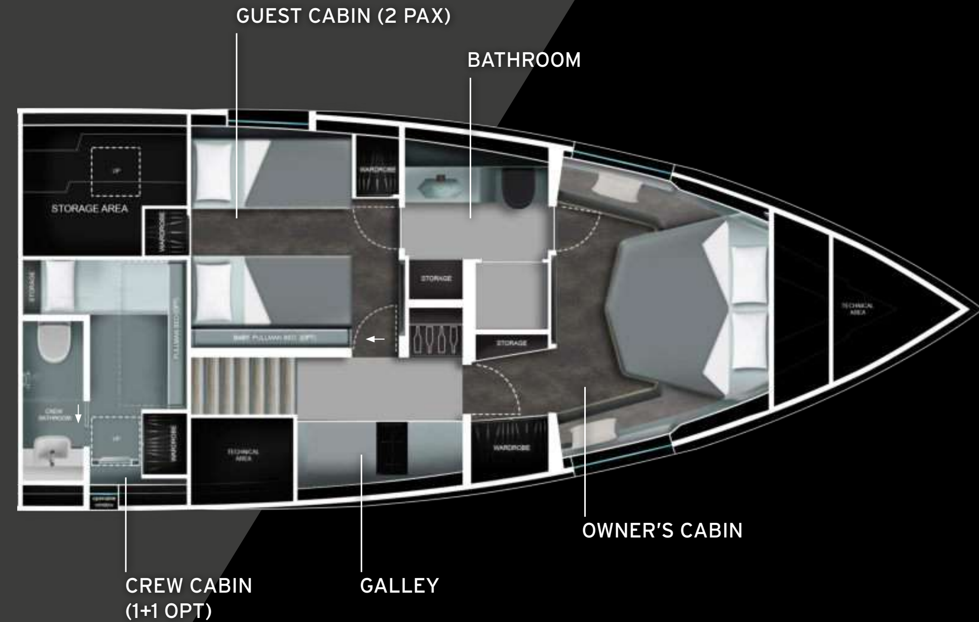
TWO CABINS LAYOUT 4+1 GUEST
