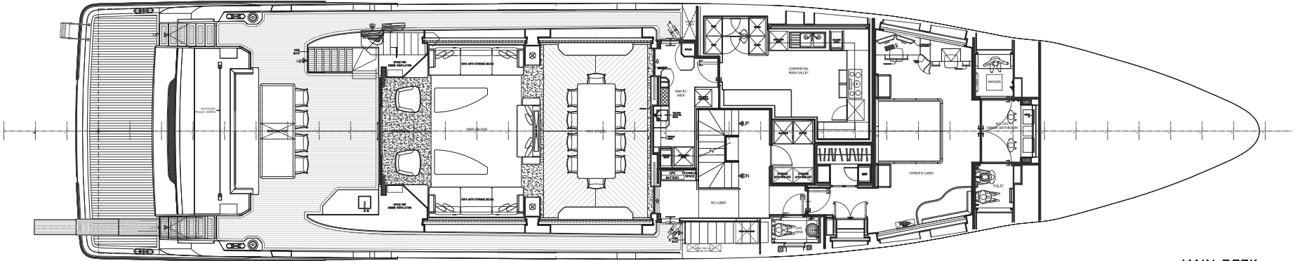
MAIN DECK
