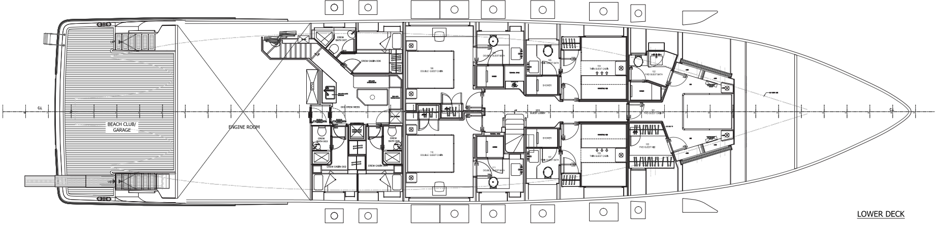
LOWER DECK
