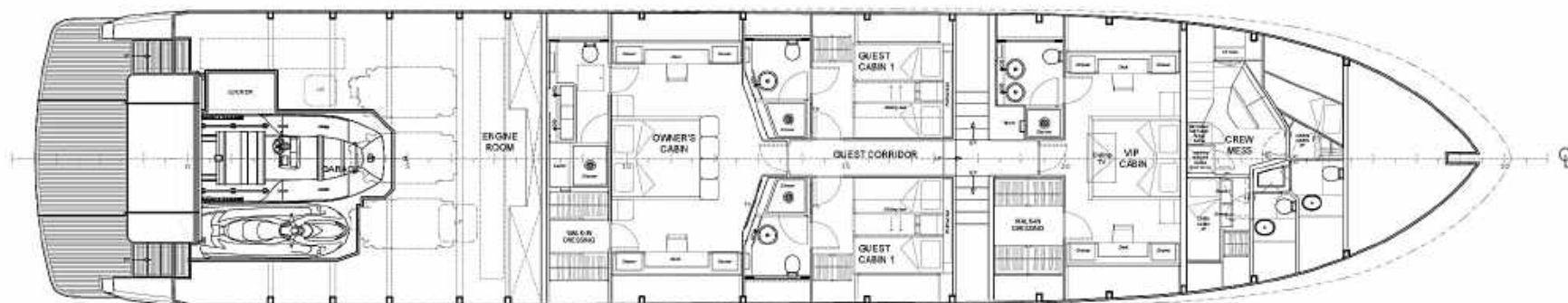
LOWER DECK
