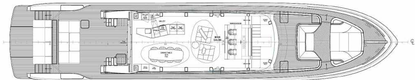
MAIN DECK
